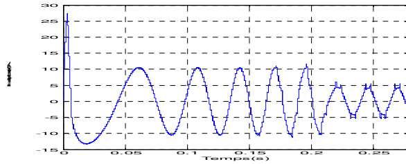
Figure 10: Stator Current of Phase \alpha , Case: (DTNC)
